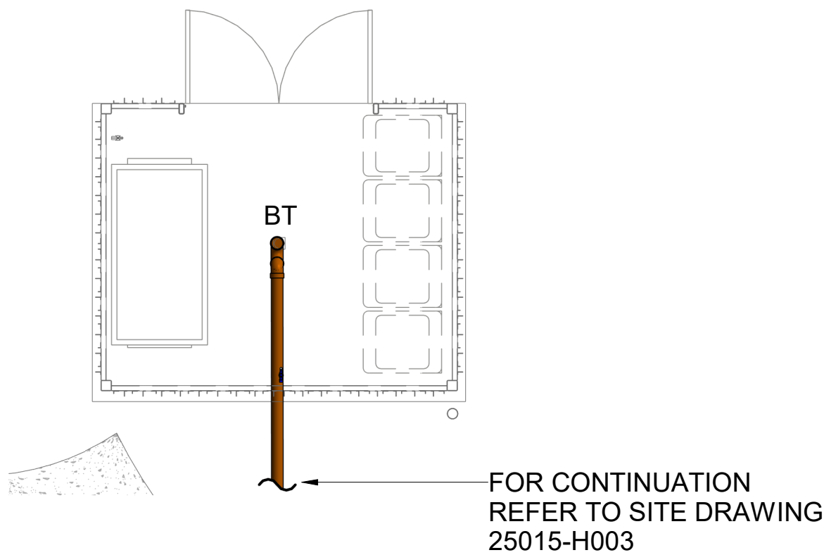
NBC BINWASH SANITARY LAYOUT 1 : 50
