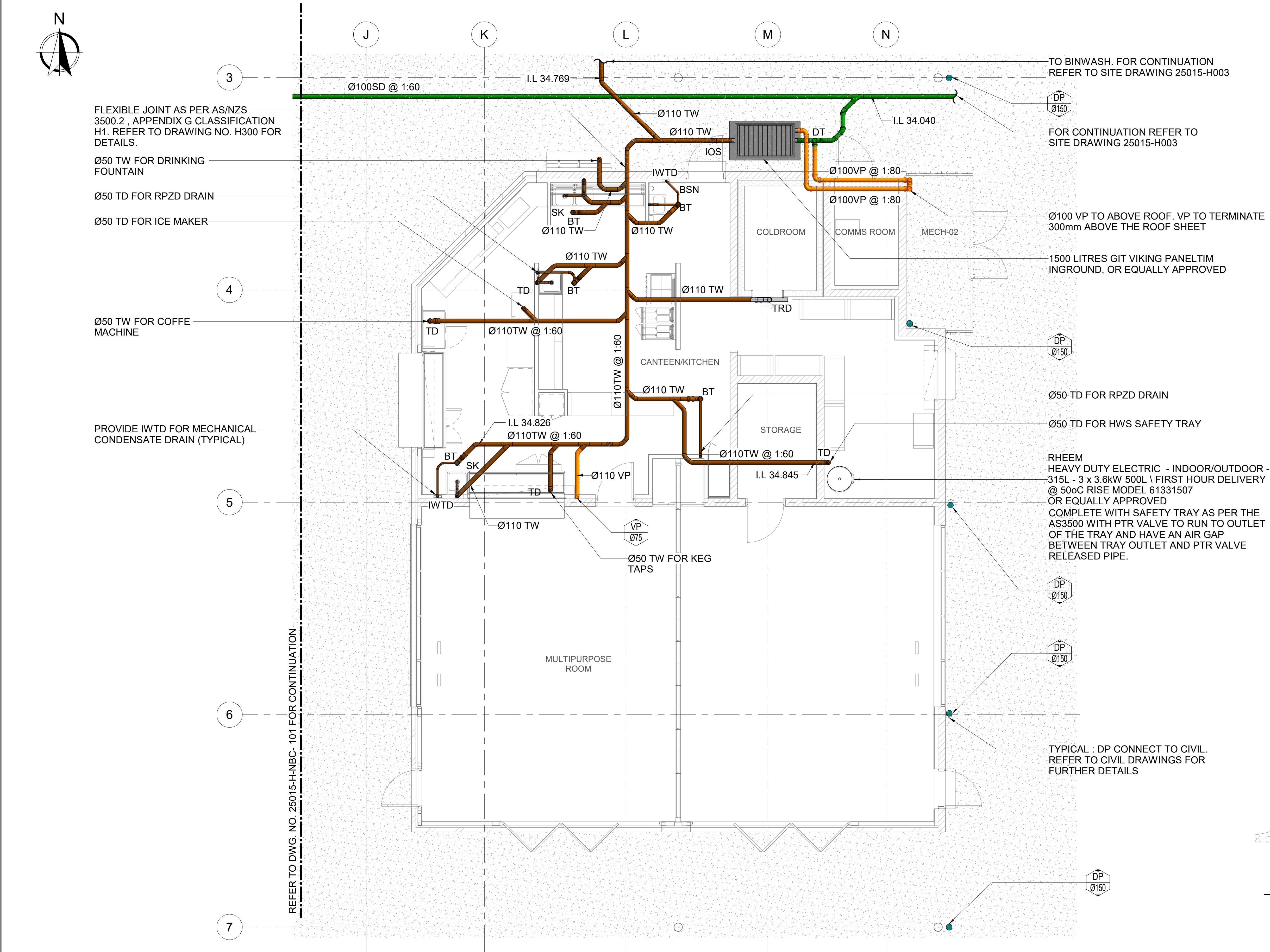
GROUND FLOOR SANITARY PLUMBING LAYOUT - PART PLAN 3 1 : 50
